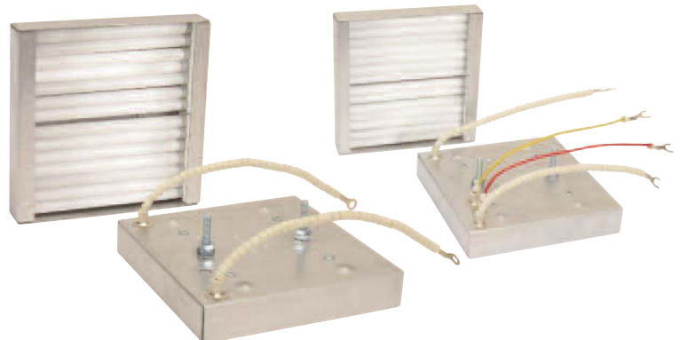
Style S – Two 10-32 Studs x 1" on centerline (Shown with Translucent Tubes and T/C)
