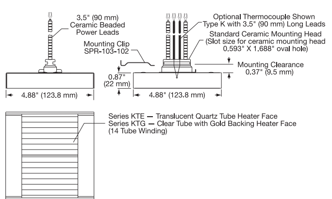
Drawing C2 – Single Head Square Heater
