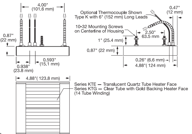
Drawing S2 – Square Heater
